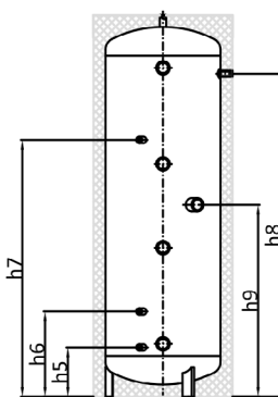
VTA-4-100-3, VTA-4-150-3
