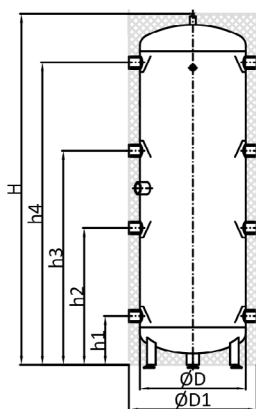
VTA-4-100-3, VTA-4-150-3
